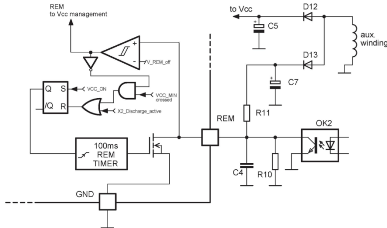
Figure 40. Simplified Block Diagram of Remote Control Input for Active ON Off-mode
